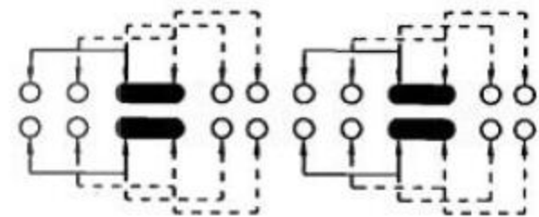
SCHEMATIC (SHORTING)
